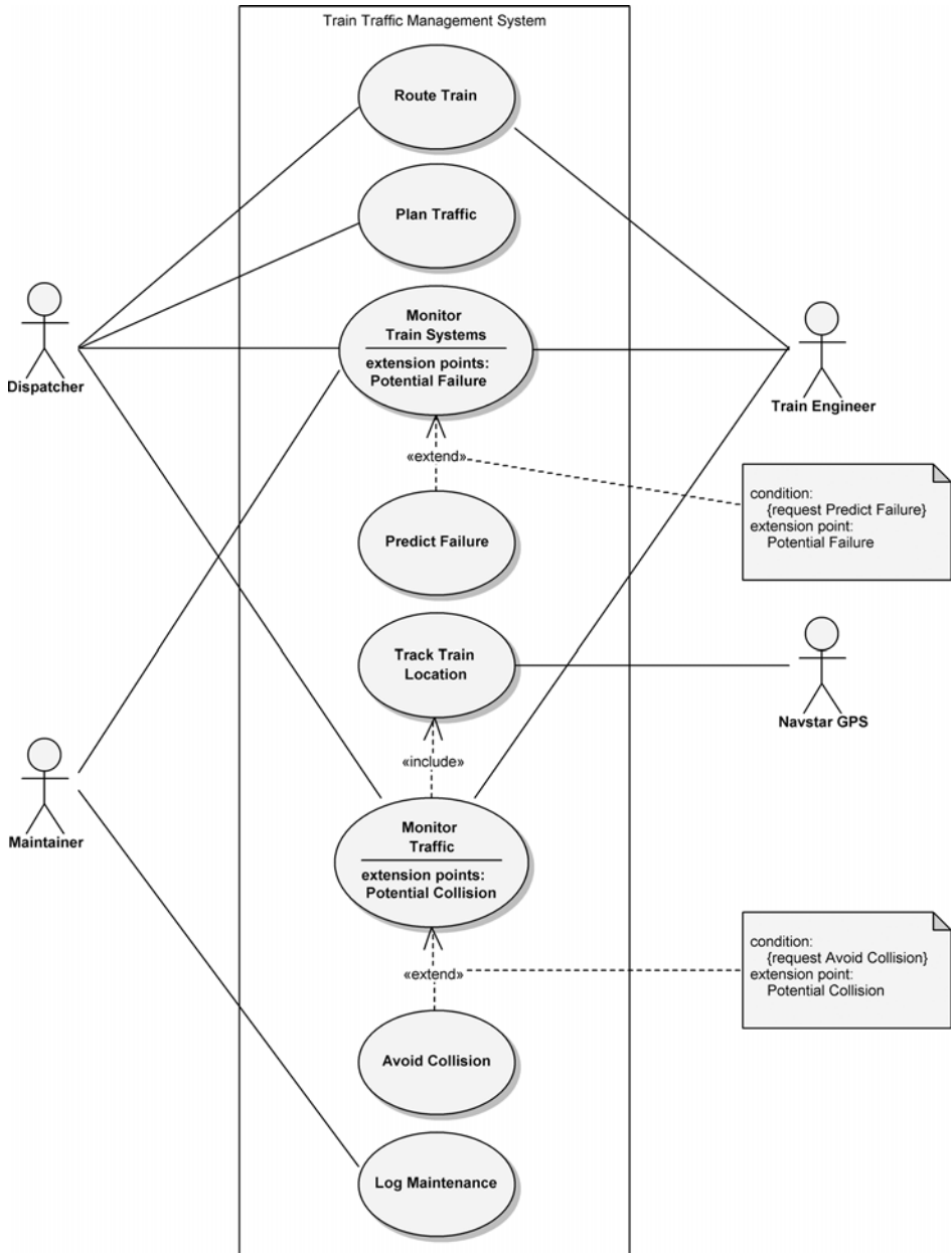
Figure 9-1 The Use Case Diagram for the Train Traffic Management System
