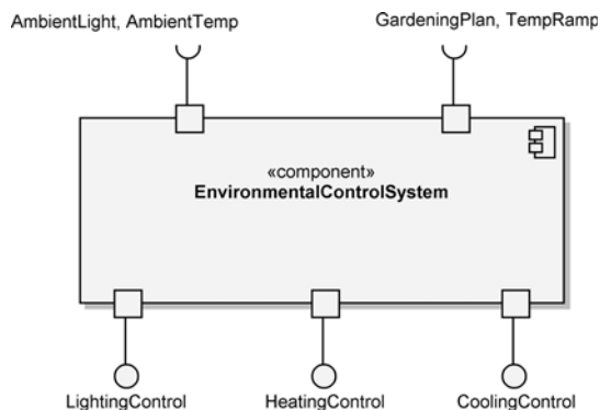
Figure 5–10 The Component Notation with Interface Grouping
